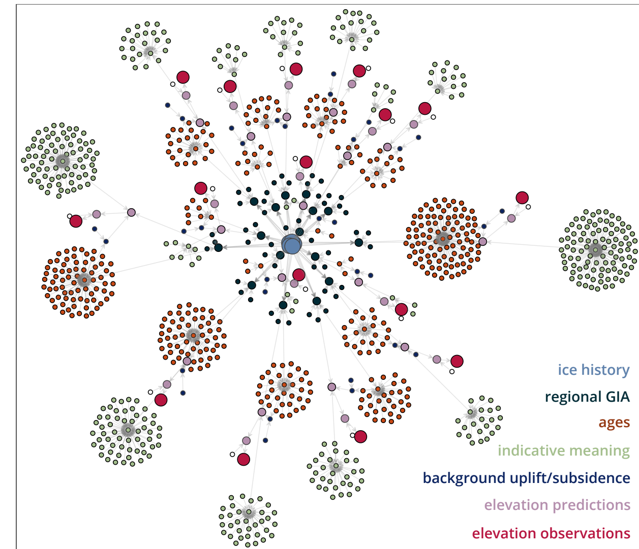
A graphical representation of a Bayesian inference model for paleo sea-level reconstructions
